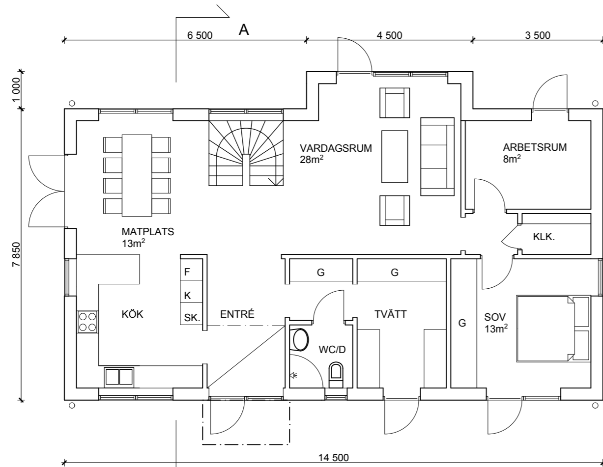
PLAN 1 104 m 2
