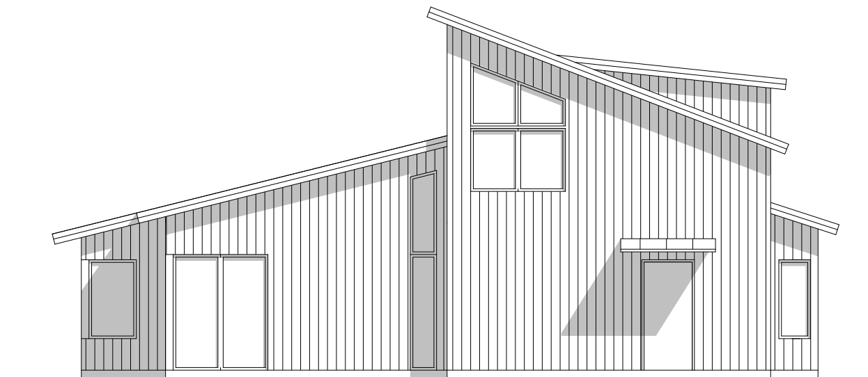
GAVELFASAD 1
